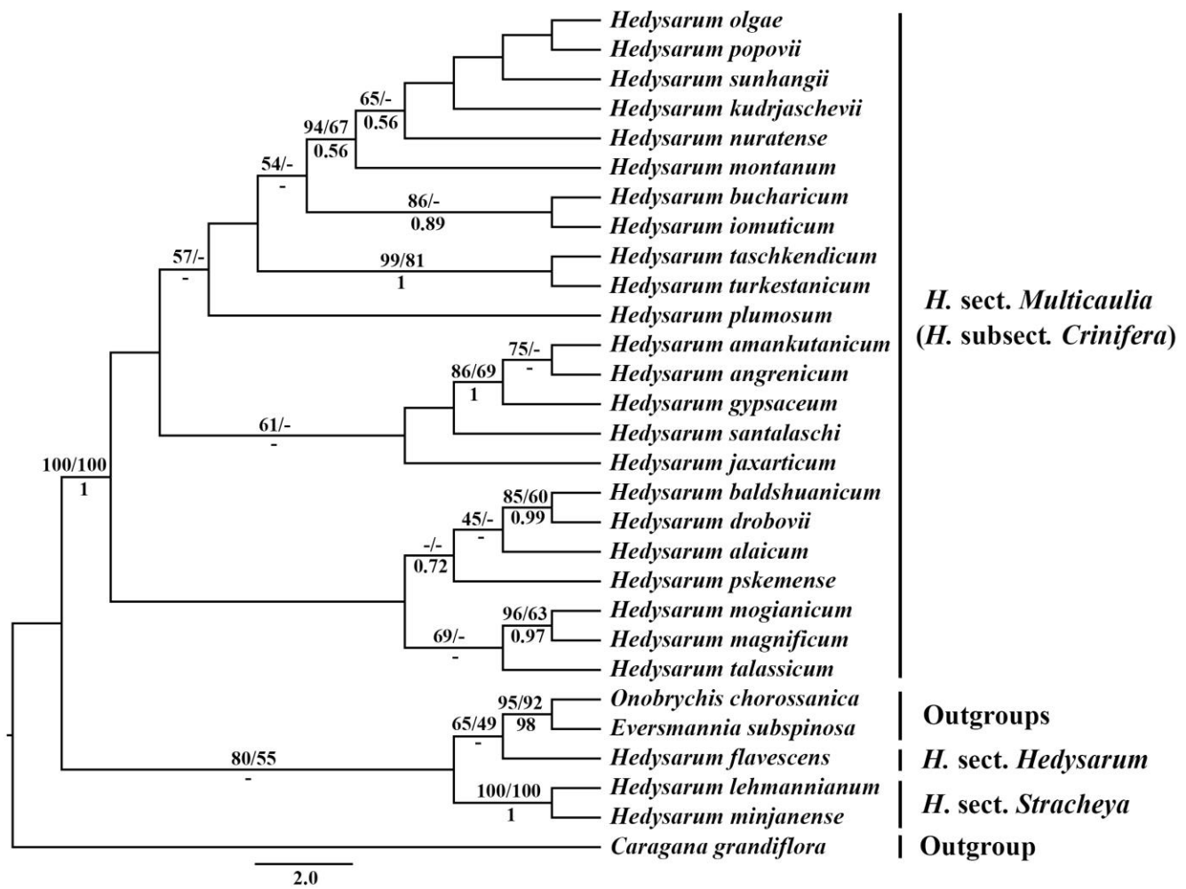
Fig. S1. Maximum likelihood tree inferred from nrDNA ITS sequences. Bootstrap values of maximum likelihood (ML) / maximum parsimony (MP) are given on each branch; Bayesian posterior probability (PP) is below branches. Only bootstrap values >45% are shown.
